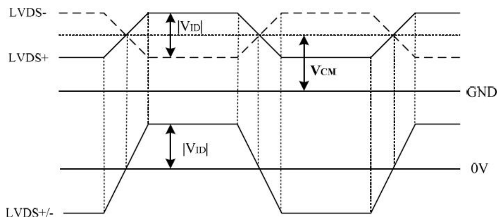
Figure 7 Voltage Definition
